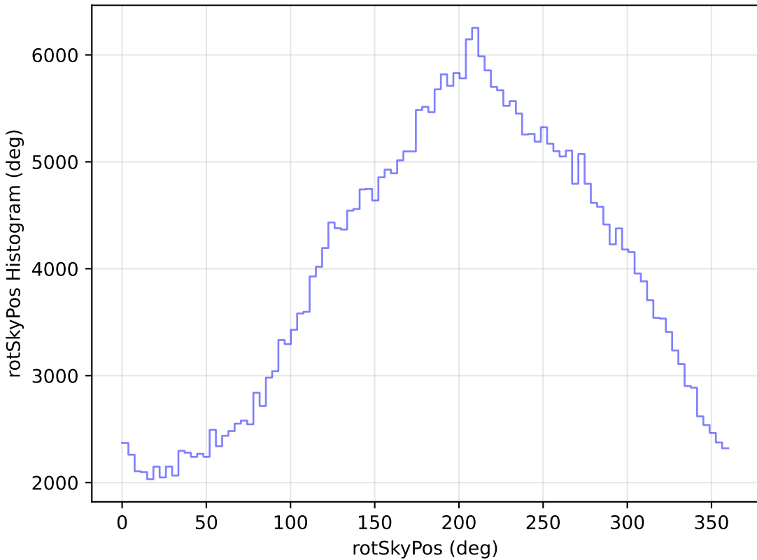
noroll_mjdp180_v3.4_10yrs All sky y band: rotSkyPos Histogram
