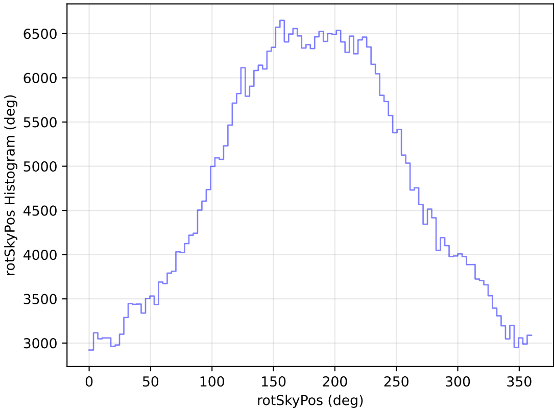
noroll_mjdp180_v3.4_10yrs All sky r band: rotSkyPos Histogram
