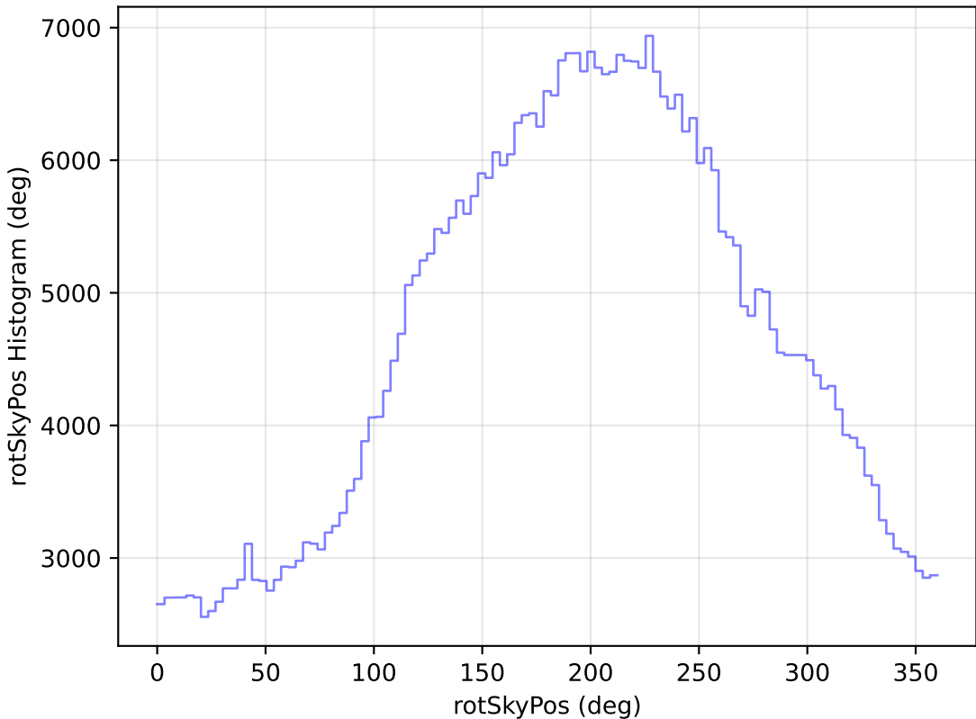
noroll_mjdp180_v3.4_10yrs All sky i band: rotSkyPos Histogram
