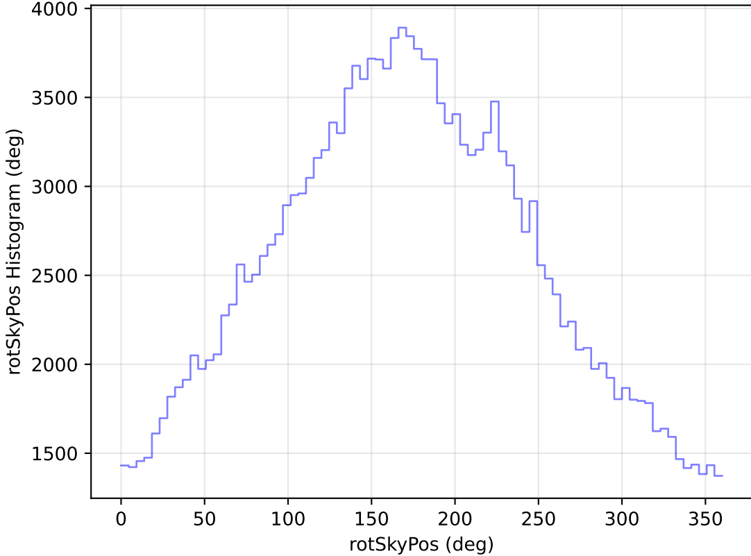
noroll_mjdp180_v3.4_10yrs All sky g band: rotSkyPos Histogram
