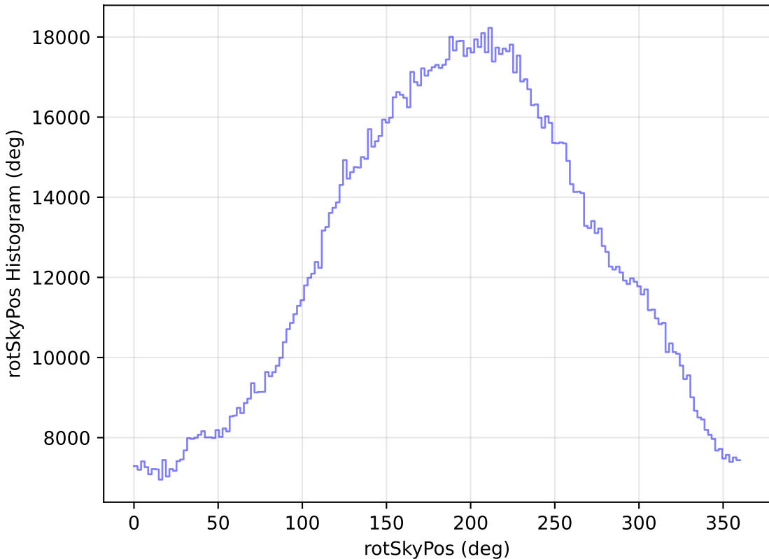
noroll_mjdp180_v3.4_10yrs All sky all bands: rotSkyPos Histogram
