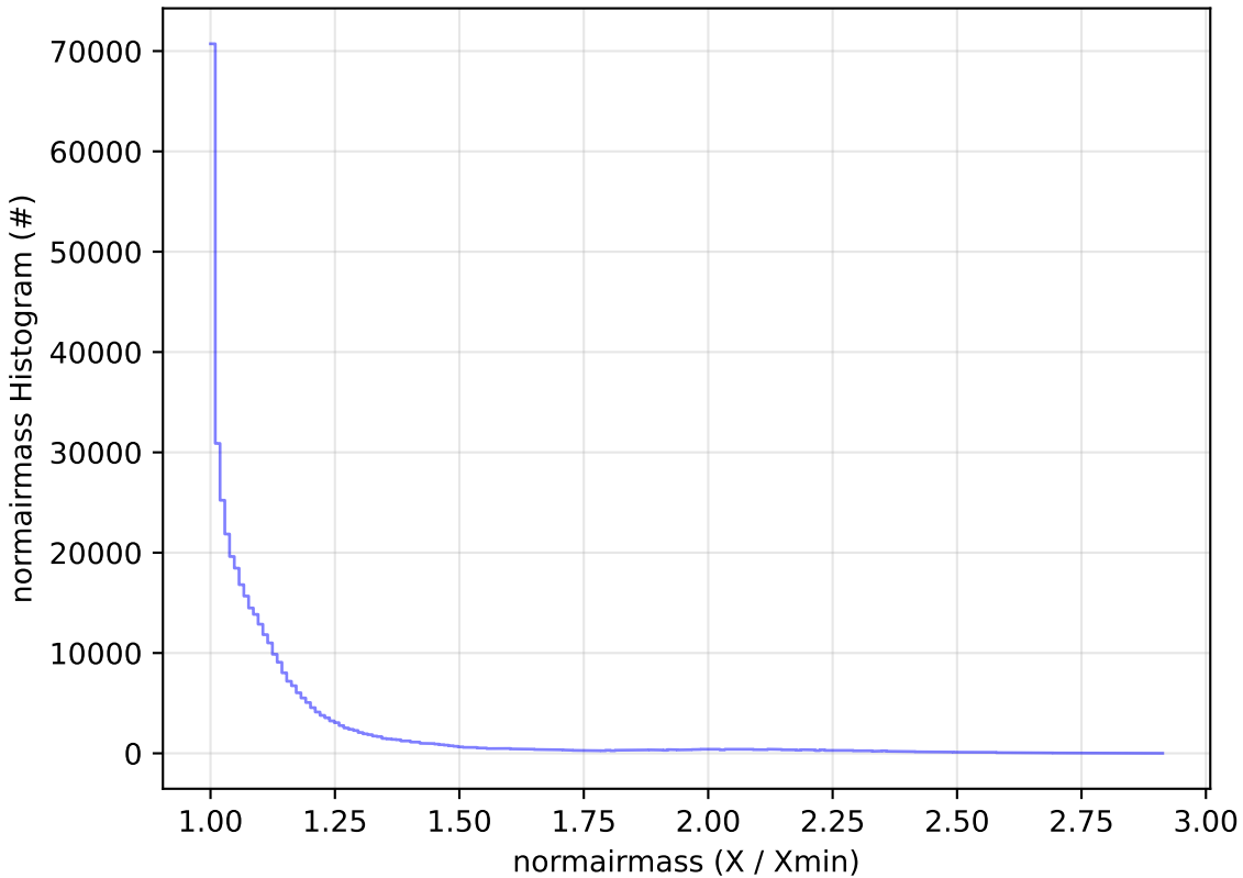
noroll_mjdp180_v3.4_10yrs WFD z band: normairmass Histogram
