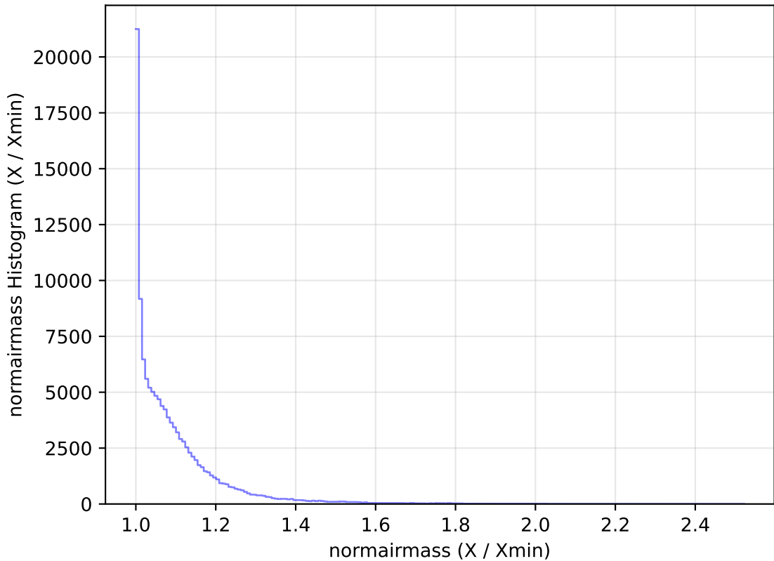
noroll_mjdp180_v3.4_10yrs WFD u band: normairmass Histogram
