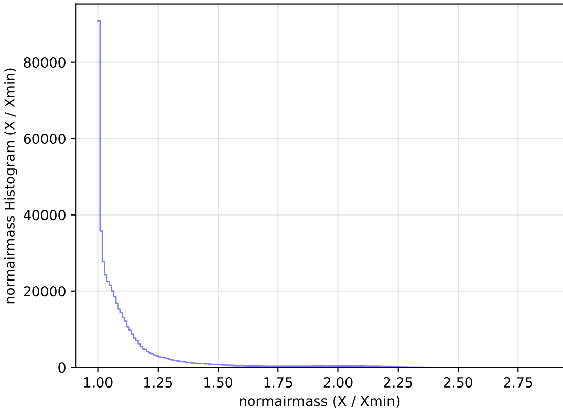
noroll_mjdp180_v3.4_10yrs WFD r band: normairmass Histogram
