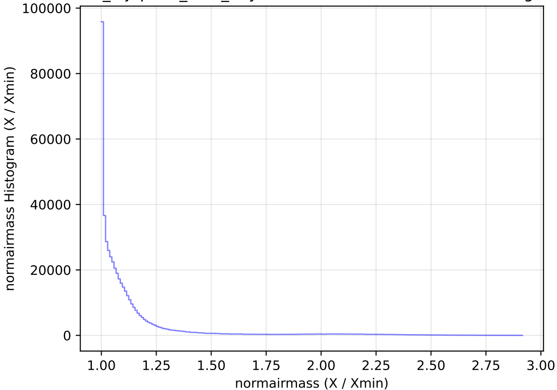
noroll_mjdp180_v3.4_10yrs WFD i band: normairmass Histogram
