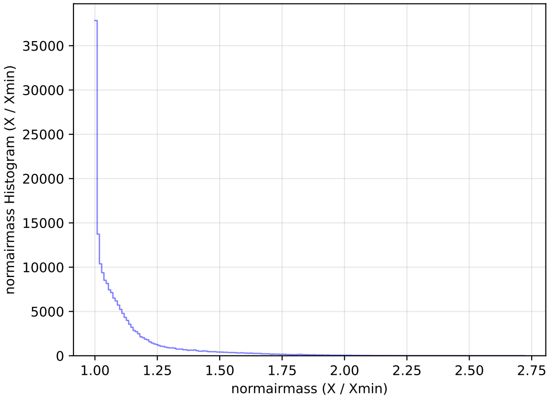
noroll_mjdp180_v3.4_10yrs WFD g band: normairmass Histogram
