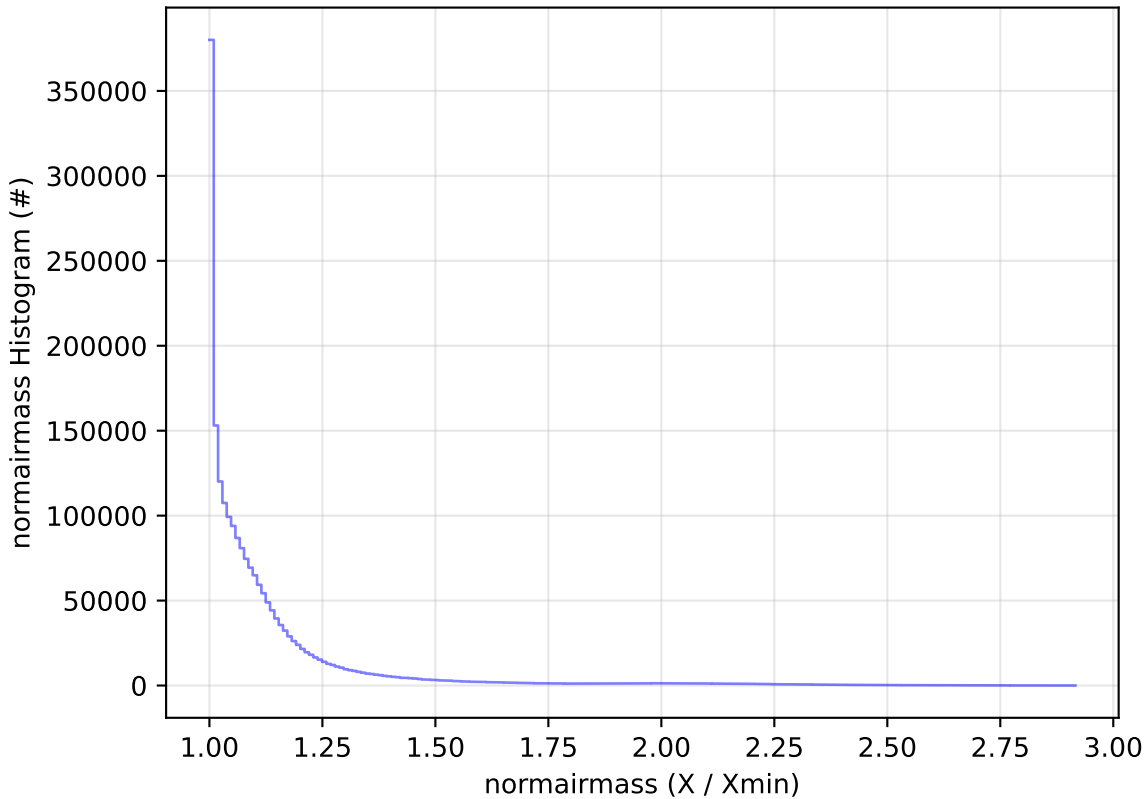
noroll_mjdp180_v3.4_10yrs WFD all bands: normairmass Histogram
