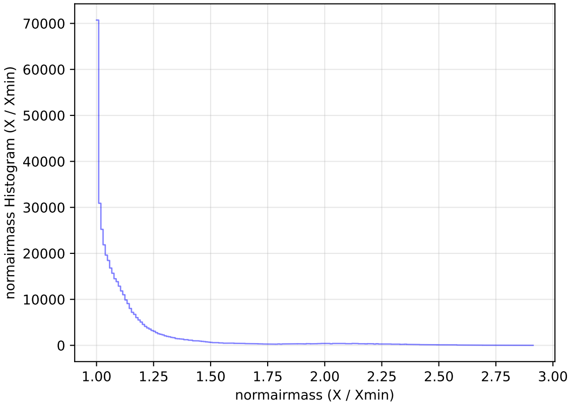
noroll_mjdp180_v3.4_10yrs All sky z band: normairmass Histogram
