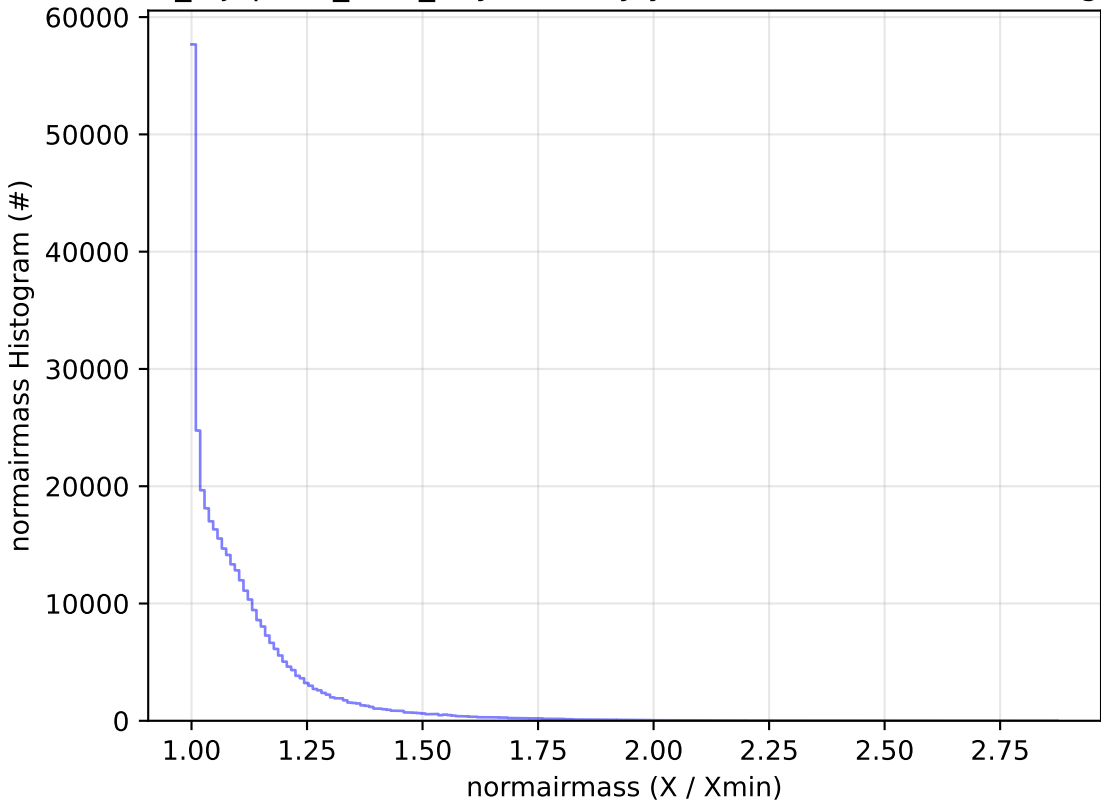
noroll_mjdp180_v3.4_10yrs All sky y band: normairmass Histogram
