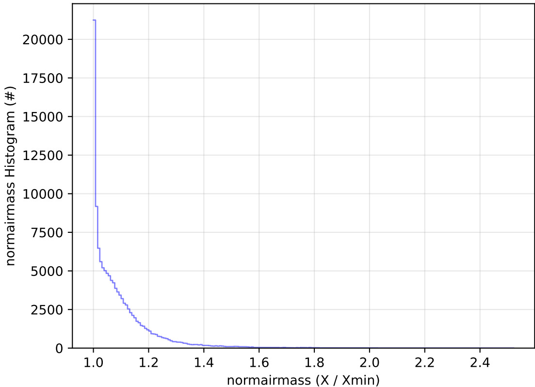
noroll_mjdp180_v3.4_10yrs All sky u band: normairmass Histogram
