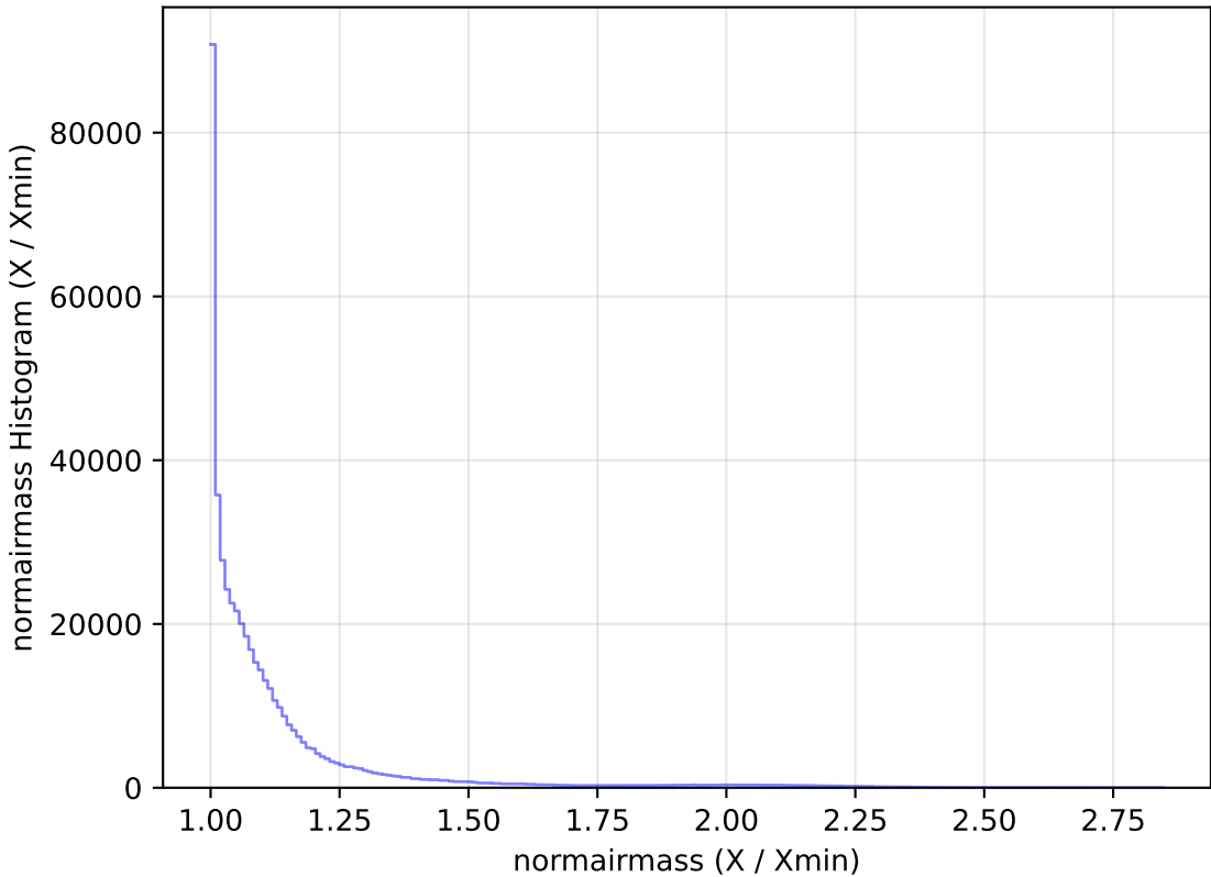
noroll_mjdp180_v3.4_10yrs All sky r band: normairmass Histogram
