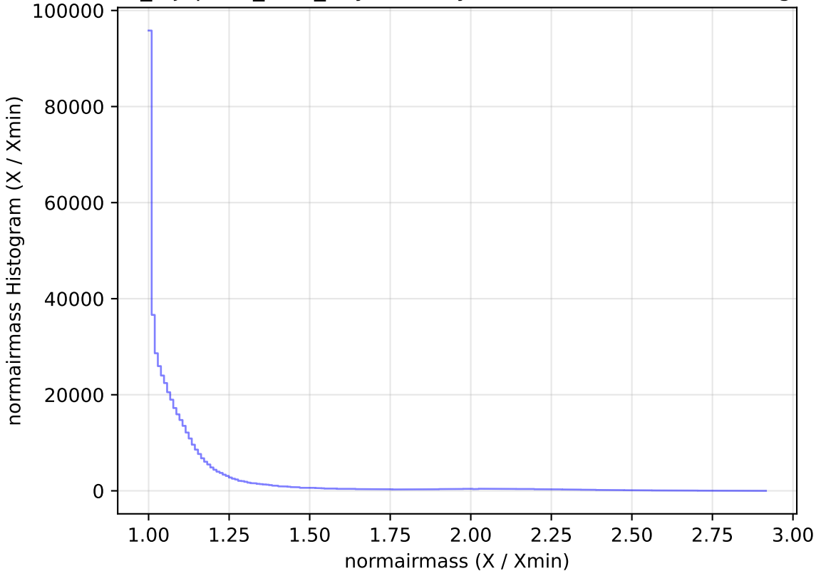
noroll_mjdp180_v3.4_10yrs All sky i band: normairmass Histogram
