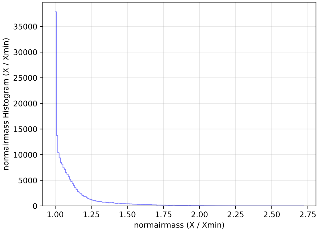
noroll_mjdp180_v3.4_10yrs All sky g band: normairmass Histogram
