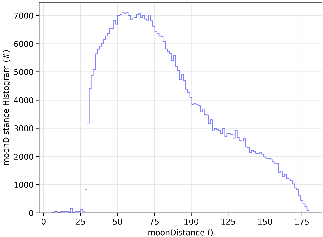
noroll_mjdp180_v3.4_10yrs WFD z band: moonDistance Histogram
