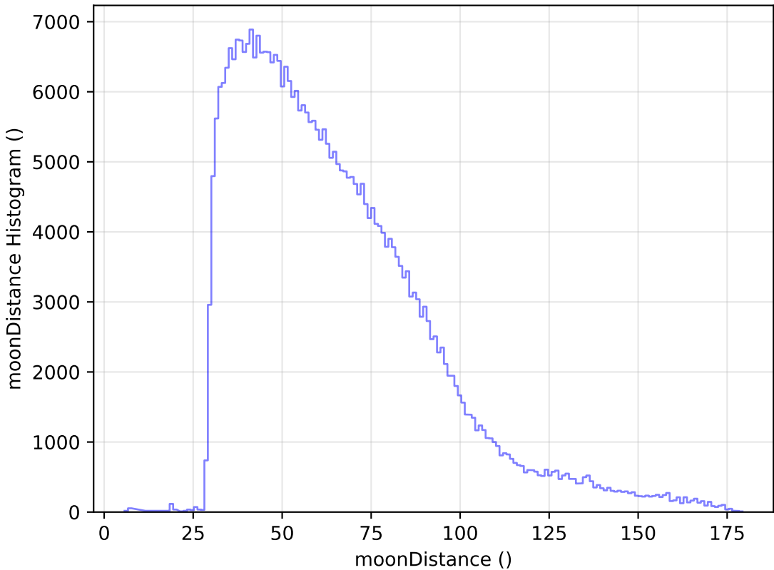
noroll_mjdp180_v3.4_10yrs WFD y band: moonDistance Histogram
