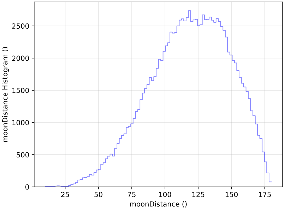
noroll_mjdp180_v3.4_10yrs WFD u band: moonDistance Histogram
