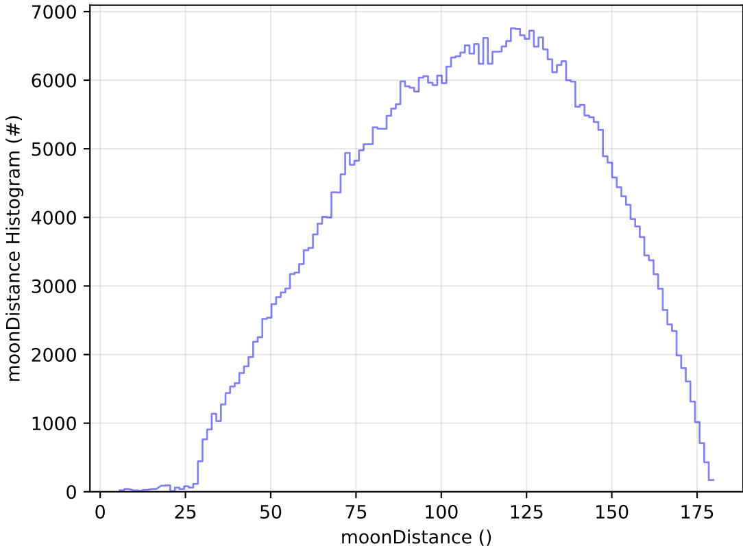
noroll_mjdp180_v3.4_10yrs WFD r band: moonDistance Histogram
