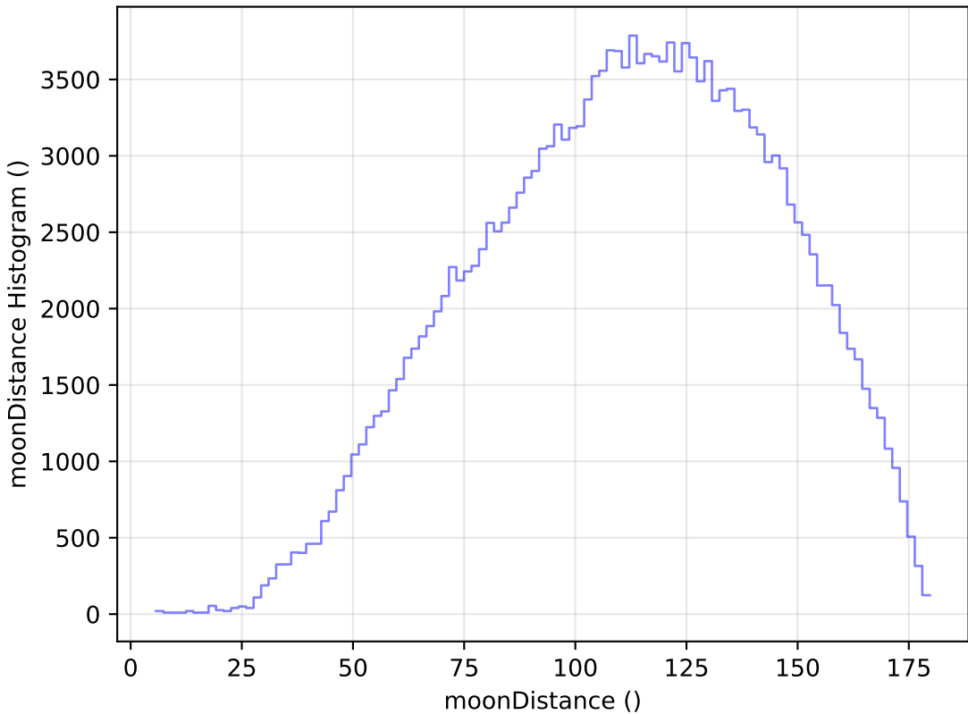
noroll_mjdp180_v3.4_10yrs WFD g band: moonDistance Histogram
