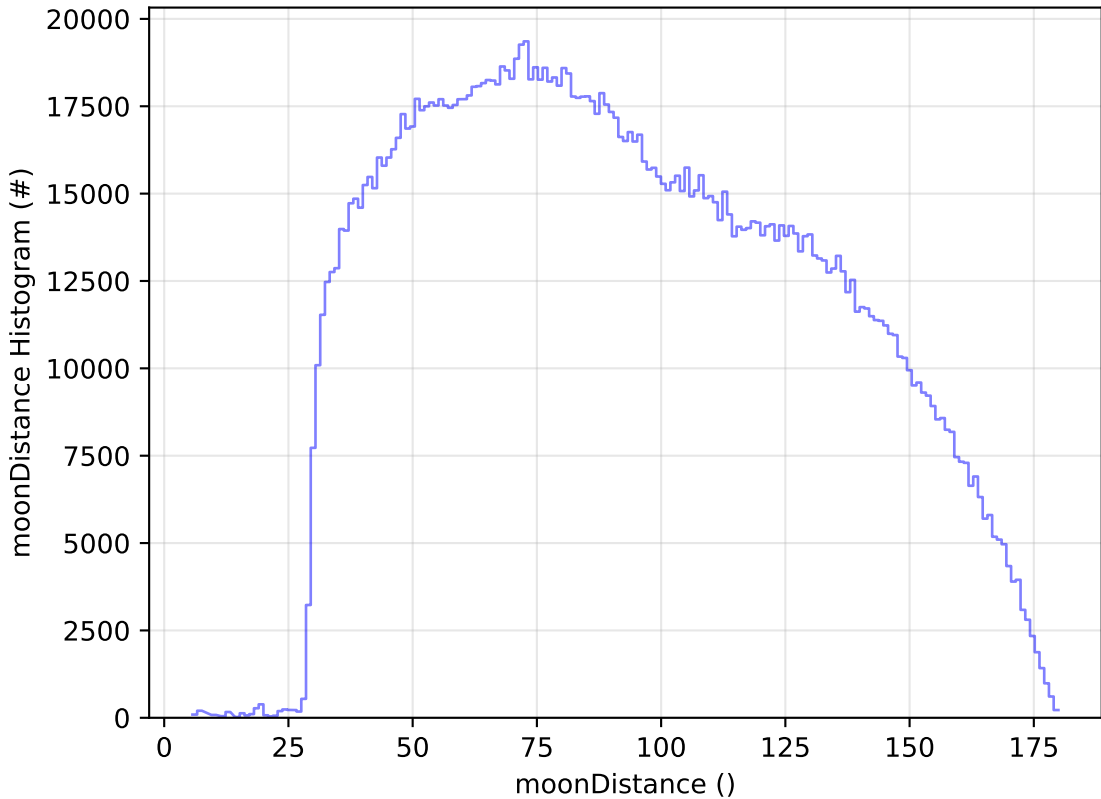
noroll_mjdp180_v3.4_10yrs WFD all bands: moonDistance Histogram
