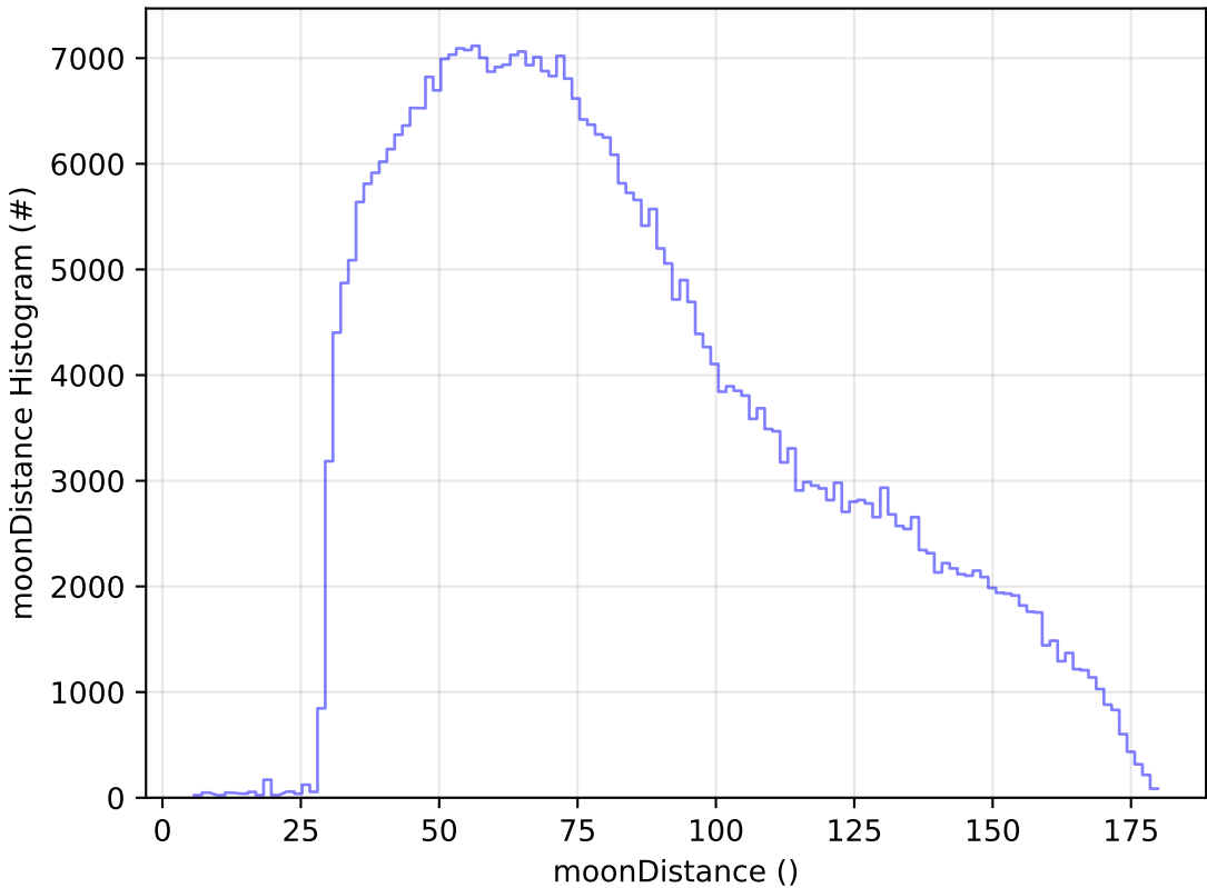
noroll_mjdp180_v3.4_10yrs All sky z band: moonDistance Histogram
