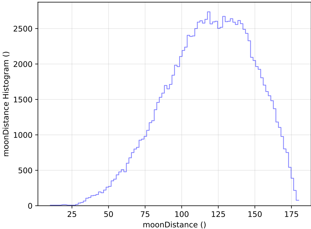
noroll_mjdp180_v3.4_10yrs All sky u band: moonDistance Histogram
