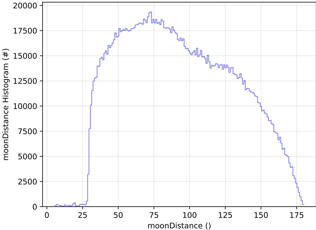
noroll_mjdp180_v3.4_10yrs All sky all bands: moonDistance Histogram
