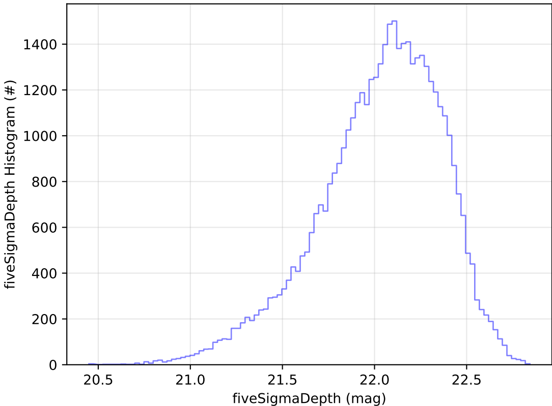
noroll_mjdp180_v3.4_10yrs Yr 1 y band: fiveSigmaDepth Histogram
