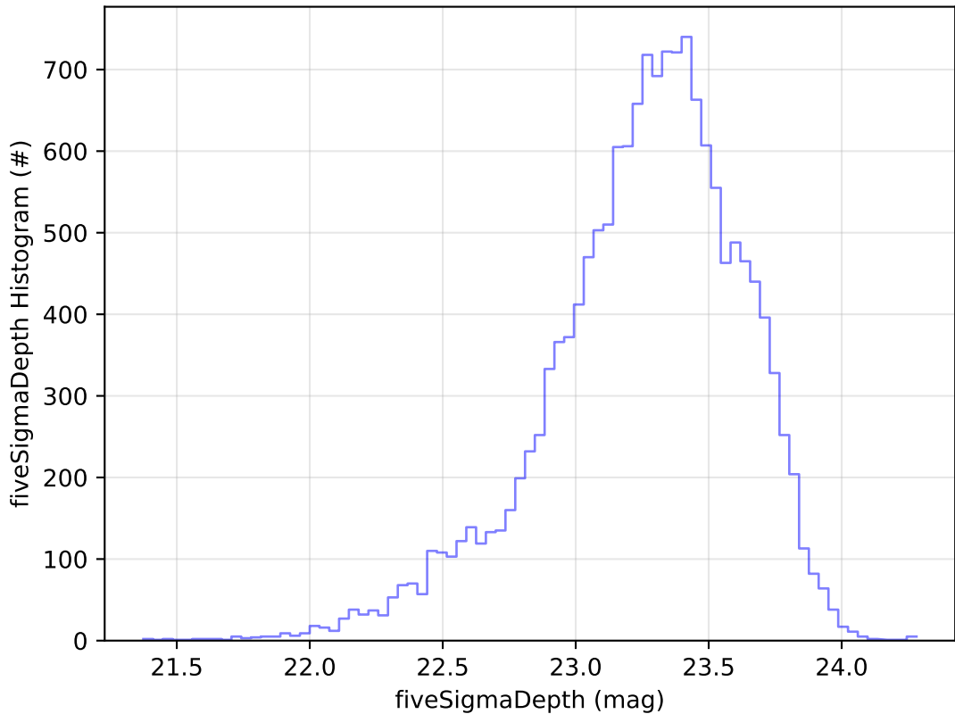
noroll_mjdp180_v3.4_10yrs Yr 1 u band: fiveSigmaDepth Histogram
