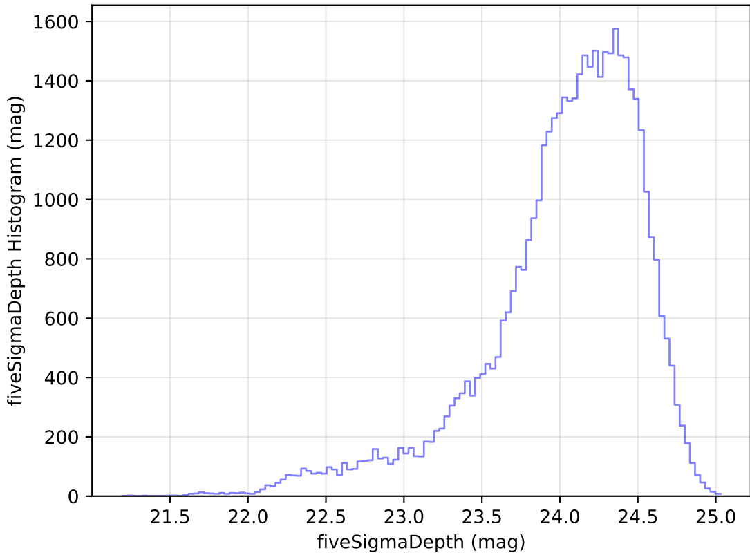
noroll_mjdp180_v3.4_10yrs Yr 1 r band: fiveSigmaDepth Histogram
