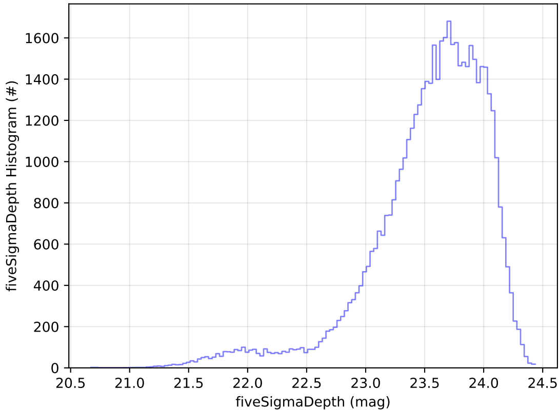
noroll_mjdp180_v3.4_10yrs Yr 1 i band: fiveSigmaDepth Histogram
