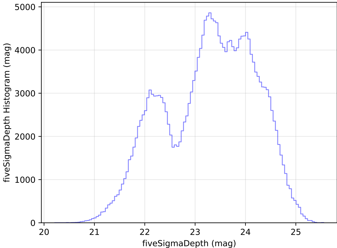
noroll_mjdp180_v3.4_10yrs Yr 1 all bands: fiveSigmaDepth Histogram
