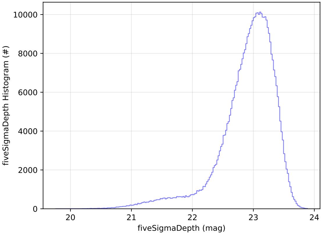
noroll_mjdp180_v3.4_10yrs WFD z band: fiveSigmaDepth Histogram
