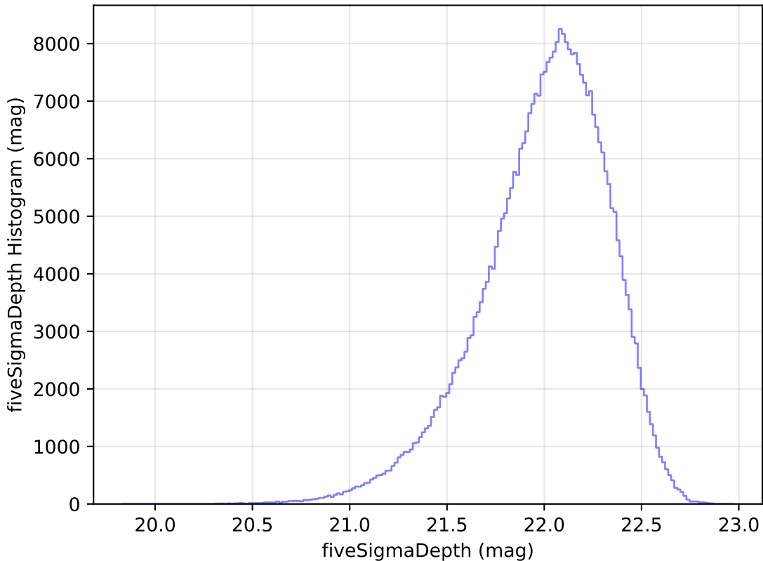
noroll_mjdp180_v3.4_10yrs WFD y band: fiveSigmaDepth Histogram
