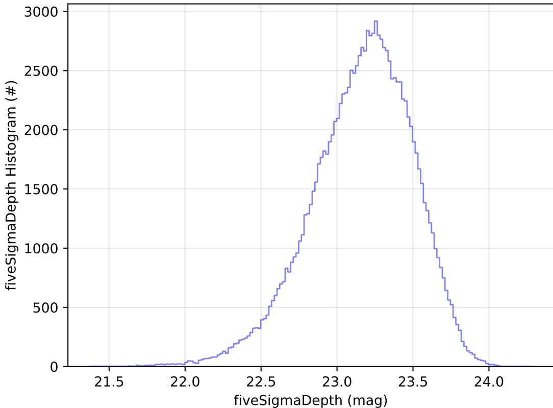
noroll_mjdp180_v3.4_10yrs WFD u band: fiveSigmaDepth Histogram
