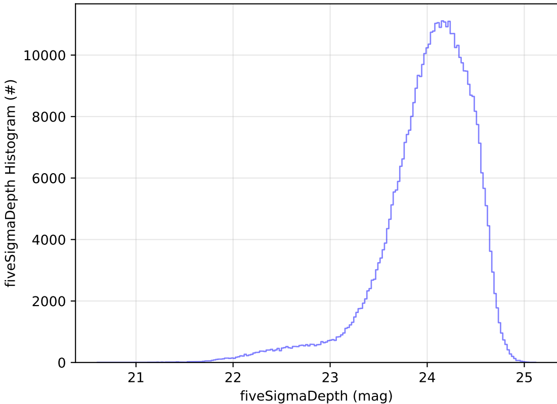
noroll_mjdp180_v3.4_10yrs WFD r band: fiveSigmaDepth Histogram
