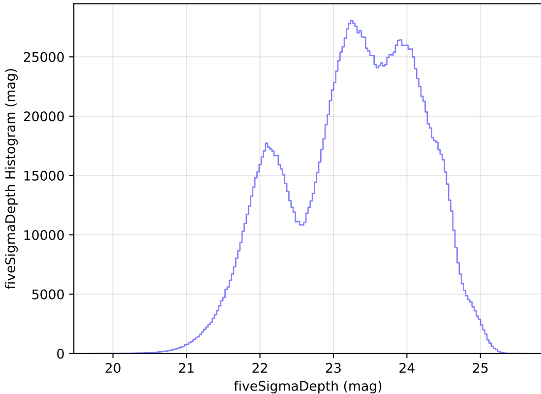
noroll_mjdp180_v3.4_10yrs WFD all bands: fiveSigmaDepth Histogram
