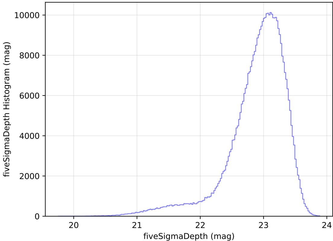
noroll_mjdp180_v3.4_10yrs All sky z band: fiveSigmaDepth Histogram
