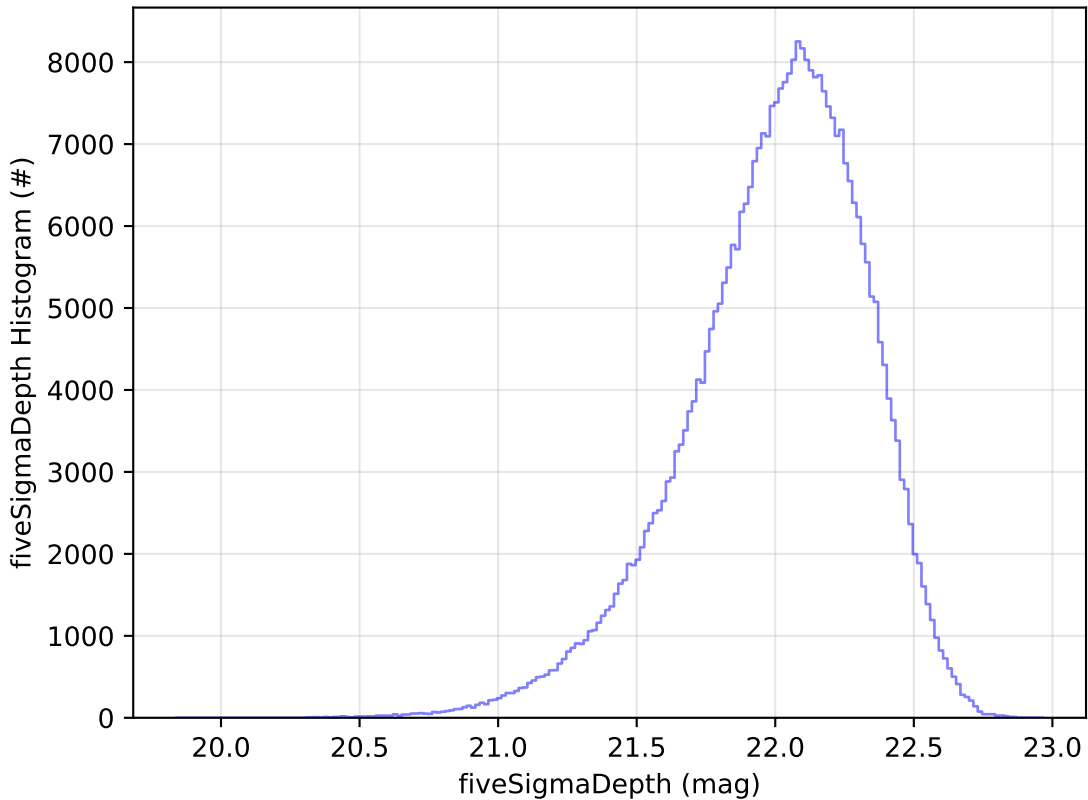
noroll_mjdp180_v3.4_10yrs All sky y band: fiveSigmaDepth Histogram
