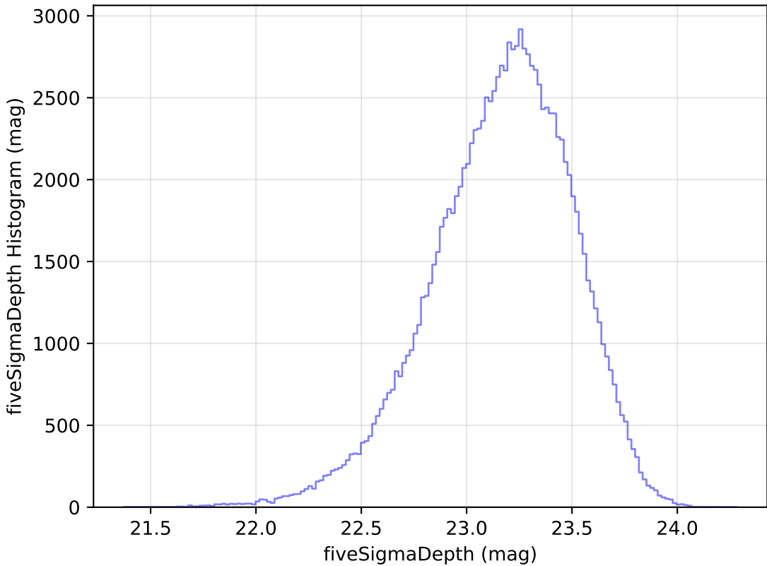
noroll_mjdp180_v3.4_10yrs All sky u band: fiveSigmaDepth Histogram
