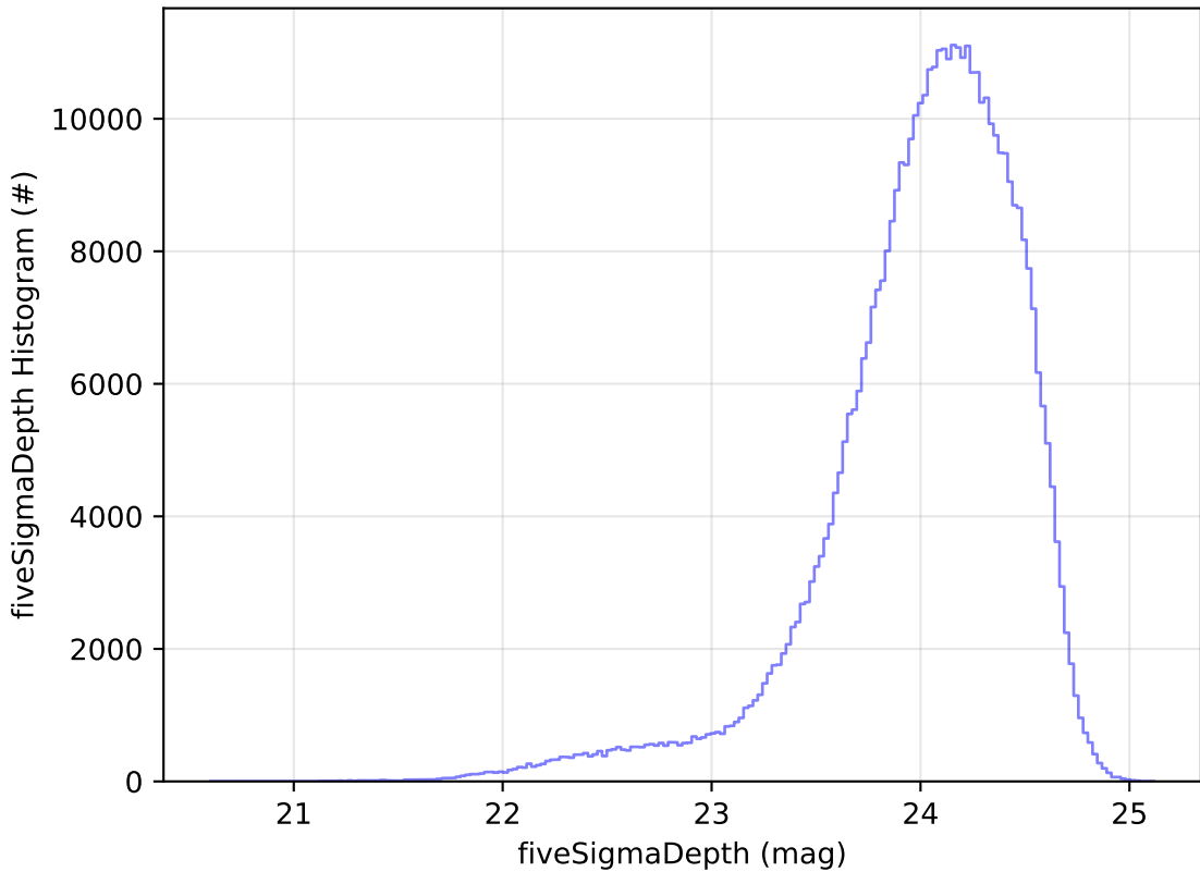
noroll_mjdp180_v3.4_10yrs All sky r band: fiveSigmaDepth Histogram
