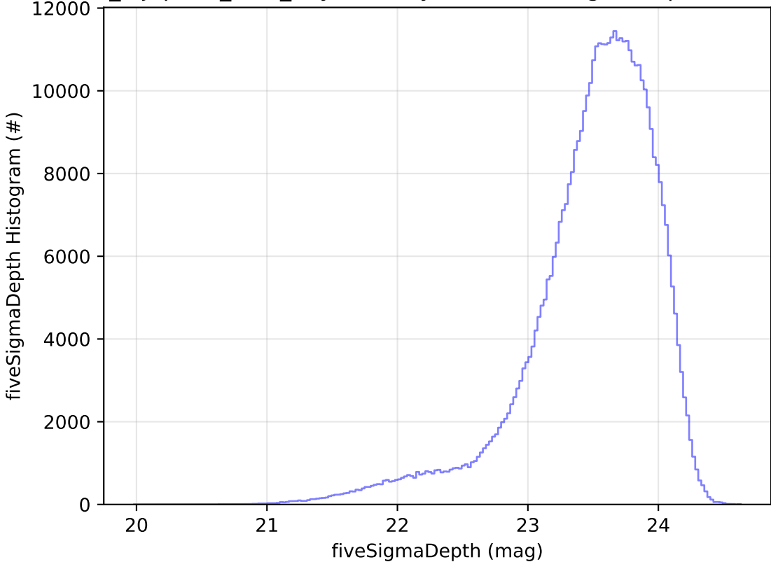
noroll_mjdp180_v3.4_10yrs All sky i band: fiveSigmaDepth Histogram
