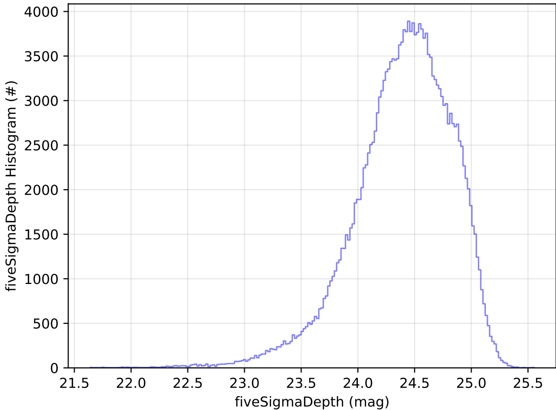
noroll_mjdp180_v3.4_10yrs All sky g band: fiveSigmaDepth Histogram
