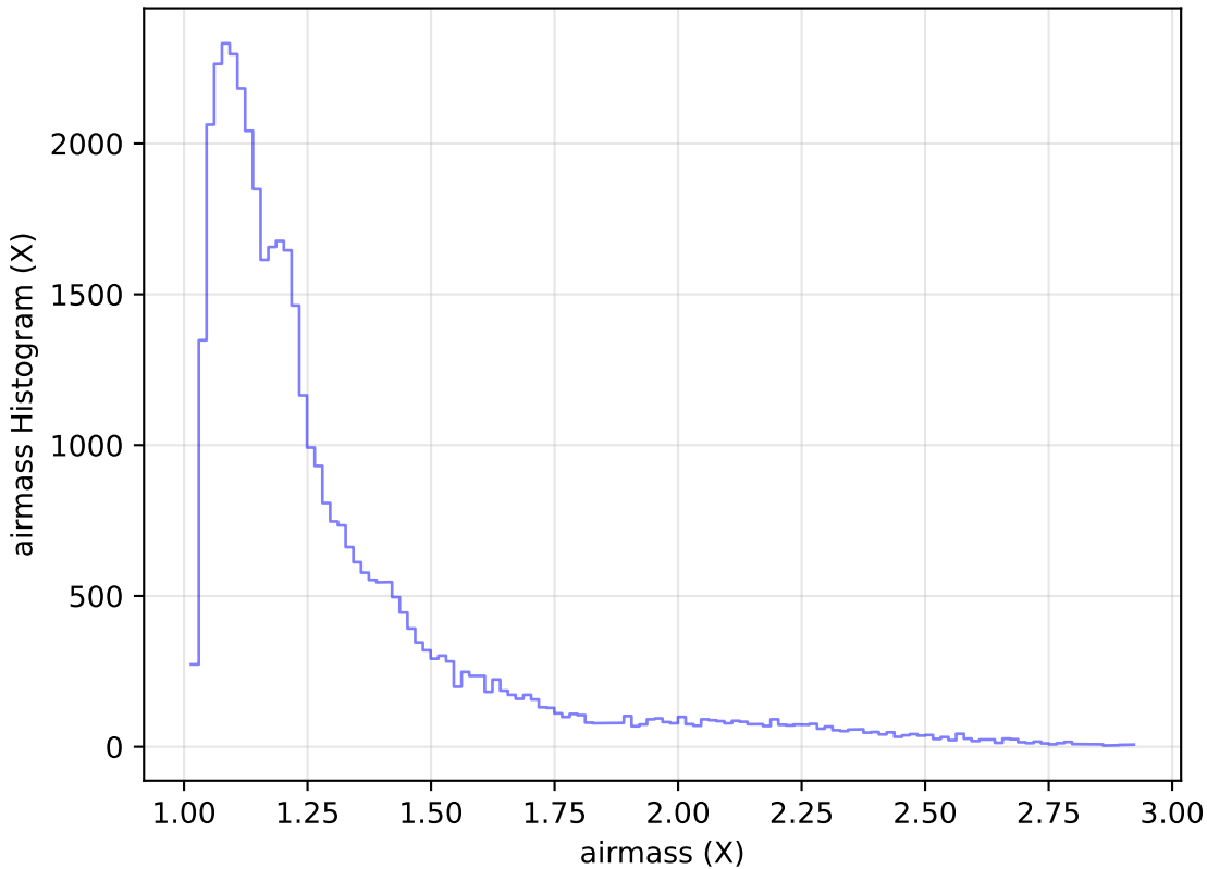
noroll_mjdp180_v3.4_10yrs Yr 1 z band: airmass Histogram
