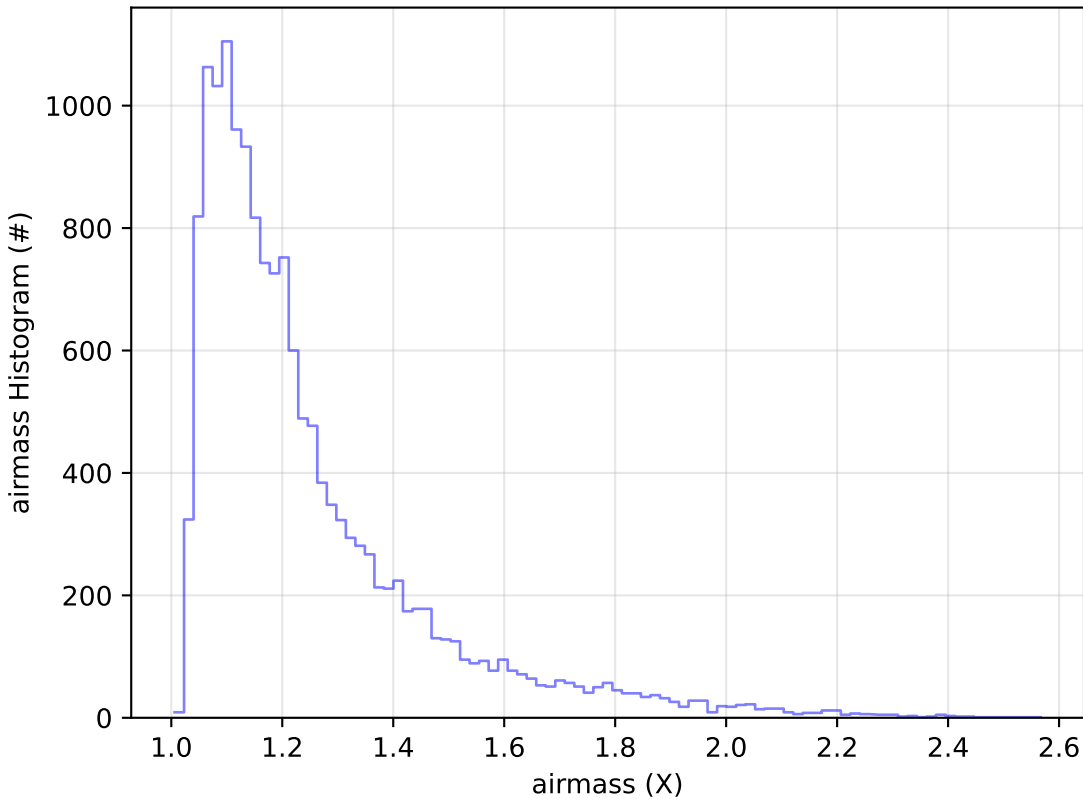
noroll_mjdp180_v3.4_10yrs Yr 1 u band: airmass Histogram
