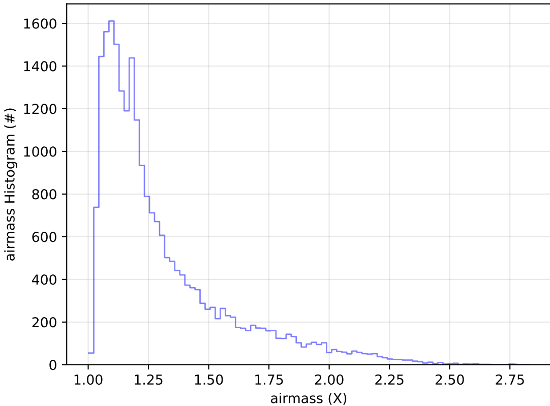
noroll_mjdp180_v3.4_10yrs Yr 1 g band: airmass Histogram
