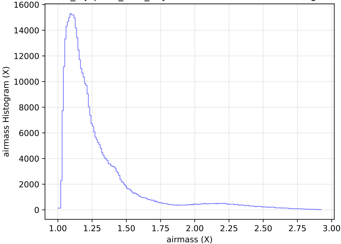
noroll_mjdp180_v3.4_10yrs WFD z band: airmass Histogram
