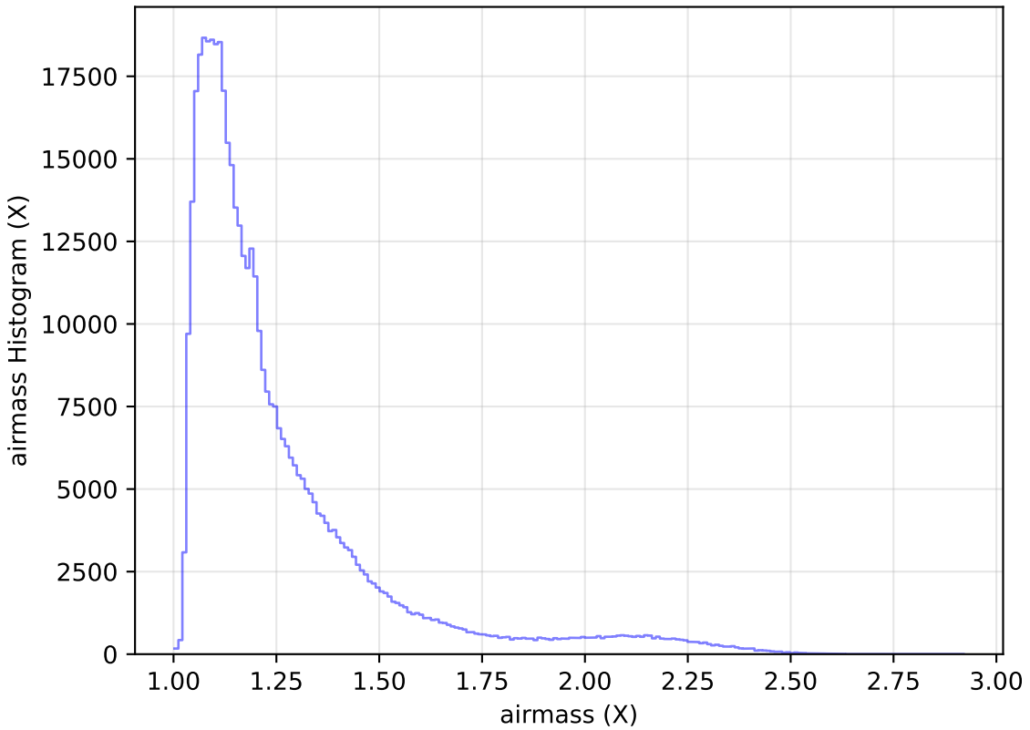
noroll_mjdp180_v3.4_10yrs WFD r band: airmass Histogram
