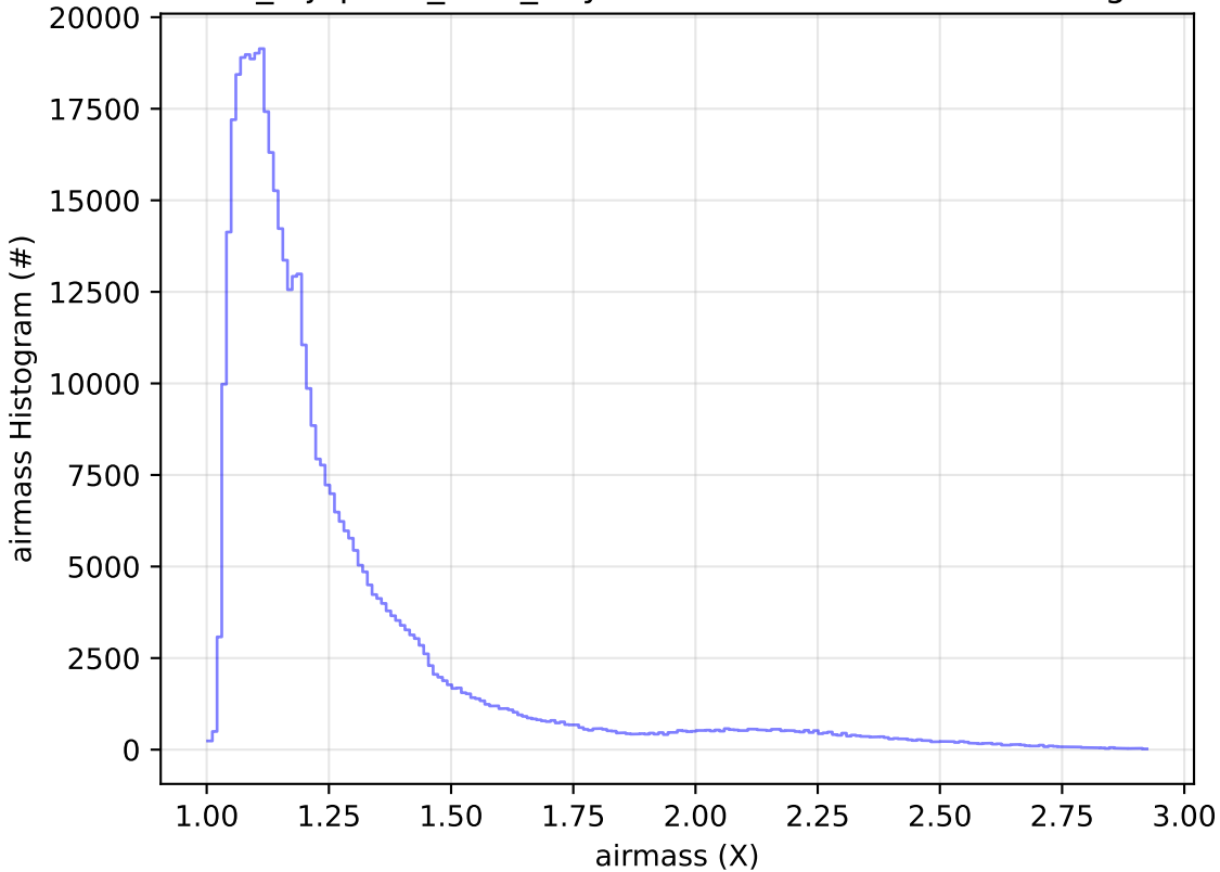
noroll_mjdp180_v3.4_10yrs WFD i band: airmass Histogram
