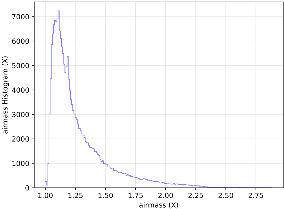
noroll_mjdp180_v3.4_10yrs WFD g band: airmass Histogram
