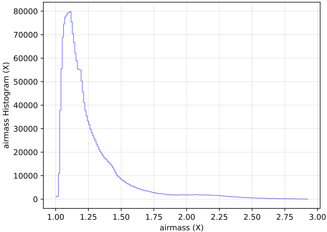
noroll_mjdp180_v3.4_10yrs WFD all bands: airmass Histogram
